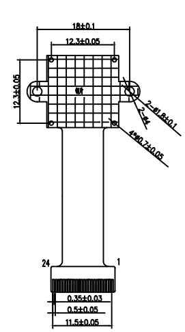
BOTTOM VIEW
